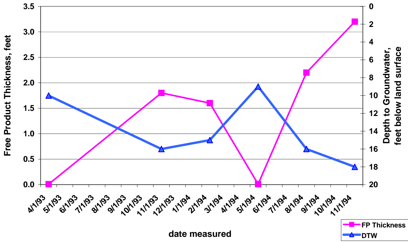
Figure C- 7 Example Graph of Depth to Groundwater and Free Product Thickness Over Time
